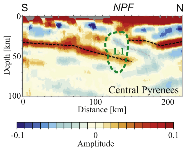
Fig. 5. a) Horizontal slice of the P velocity model from Chevrot et al., 2014 with the location of the MT sites acquired in the Central and Eastern Pyrenees (white circle). b) Comparison between Common Conversion Point (CCP) stack section from Chevrot et al., 2015 from the Central Pyrenees and the location of the L1 anomaly constrained below the Central Pyrenees (green dashed lines). Black dashed lines were associated with the Moho. NPF: North Pyrenean Fault. (For interpretation of the references to colour in this figure legend, the reader is referred to the web version of this article.)
