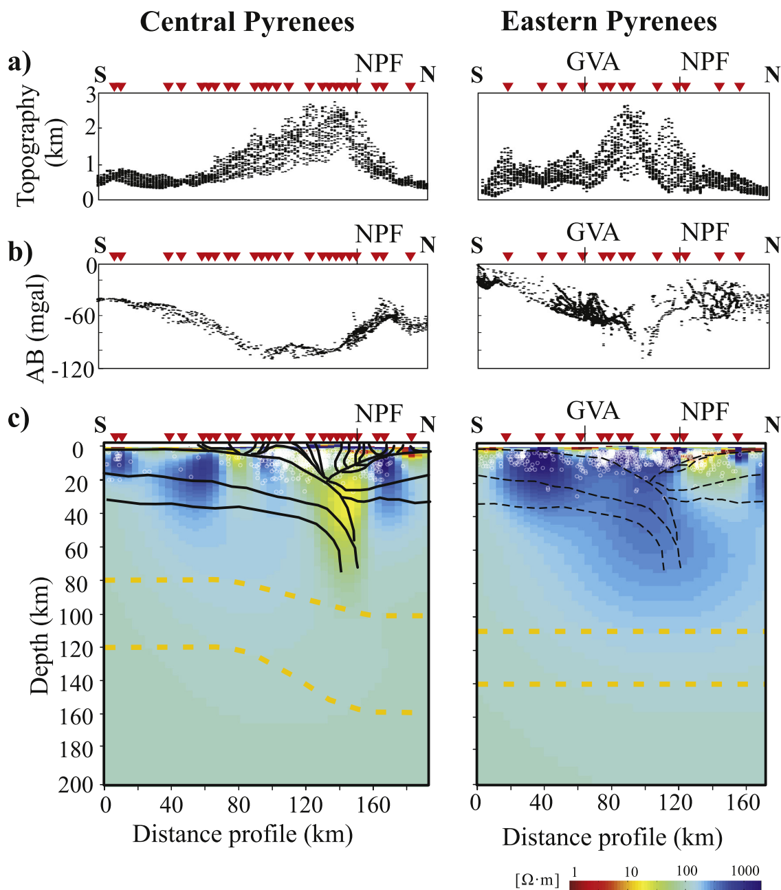
Fig. 4. a) Topography along the Central and Eastern Pyrenees MT profiles including points at \pm 0.4^\circ longitude. b) Bouguer anomaly along the Central and Eastern Pyrenees MT profiles including points at \pm 0.4^\circ longitude. c) White circles are the location of the Earthquakes below the MT profiles. Black line superimposed to the Central Pyrenees MT model is the geological interpretation based on the existent geological models (Muñoz, 1992). Black dashed lines superimposed to the Eastern Pyrenees MT model are the dipper structures of the Central Pyrenees geological interpretation using NPF as a reference point. Yellow dashed lines are the upper and lower boundaries of the eLAB from the sensitivity test. Red inverted triangles are the location of the sites. NPF: North Pyrenean Fault used as a reference point; GVA: Garrotxa Volcanic Area. (For interpretation of the references to colour in this figure legend, the reader is referred to the web version of this article.)
