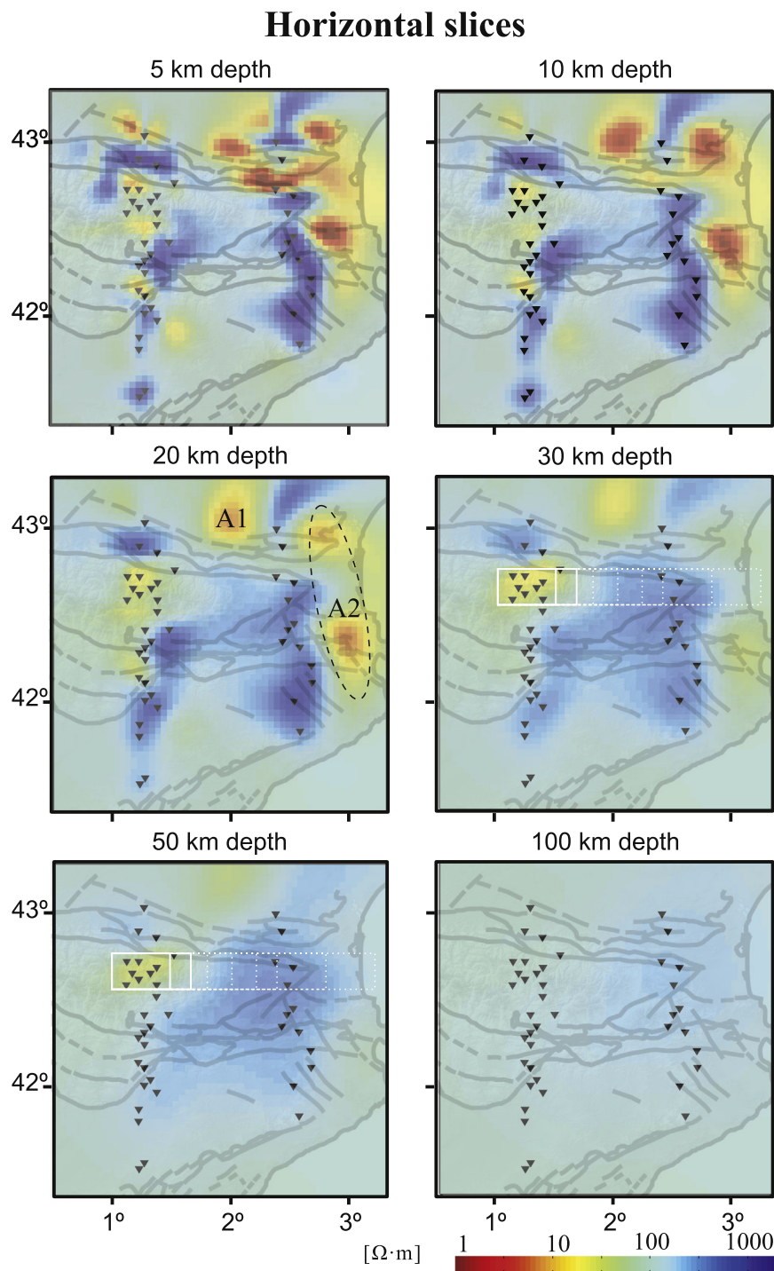
Fig. 3. Horizontal slices of the electrical resistivity model at different depths with the topography and major geological structures superimposed on top. At the slices at 20 km depth A1 and A2 are major anomalies out of the profiles. White rectangles at the slices at 30 km and 50 km depth represent the tests performed studding the eastern propagation of the conductive anomaly associated with the IBSLC (Continuous white lines are eastern edges that agree with the data; white dashed lines are tests performed propagating L1 anomaly to the east that does not agree with the data acquired at the surface).
