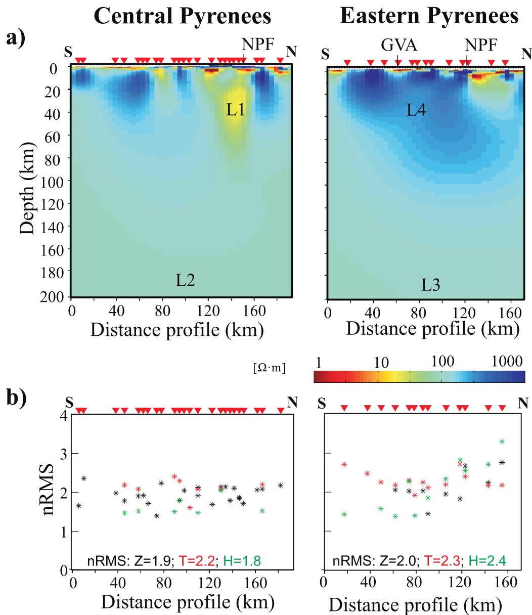
Fig. 2. a) Electrical resistivity model below the Central and Eastern Pyrenees MT profiles. L1–L4 labels showing the location of the main geoelectrical structures. Red inverted triangles at the top of the models show the location of the MT sites. NPF: North Pyrenean Fault used as a reference point; GVA: Garrotxa Volcanic Area. b) nRms between data and model responses for Z (black), T (red) and H (green) datasets at the Central and Eastern Pyrenees MT sites. (For interpretation of the references to colour in this figure legend, the reader is referred to the web version of this article.)
